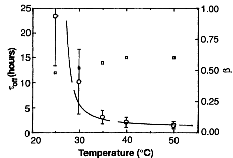
Fig. 3. Influence of temperature on desorption kinetics ( 1.0 \text{ mg ml}^{-1} PMMA in \text{CCl}_4 ). Larger error bars at the lower temperatures reflect the uncertainty of extrapolating data to times longer than the experimental time scale: (○), \tau_{\text{off}} ; and (□) \beta . Dashed line is a fit to Eq. 2 as described in text.
